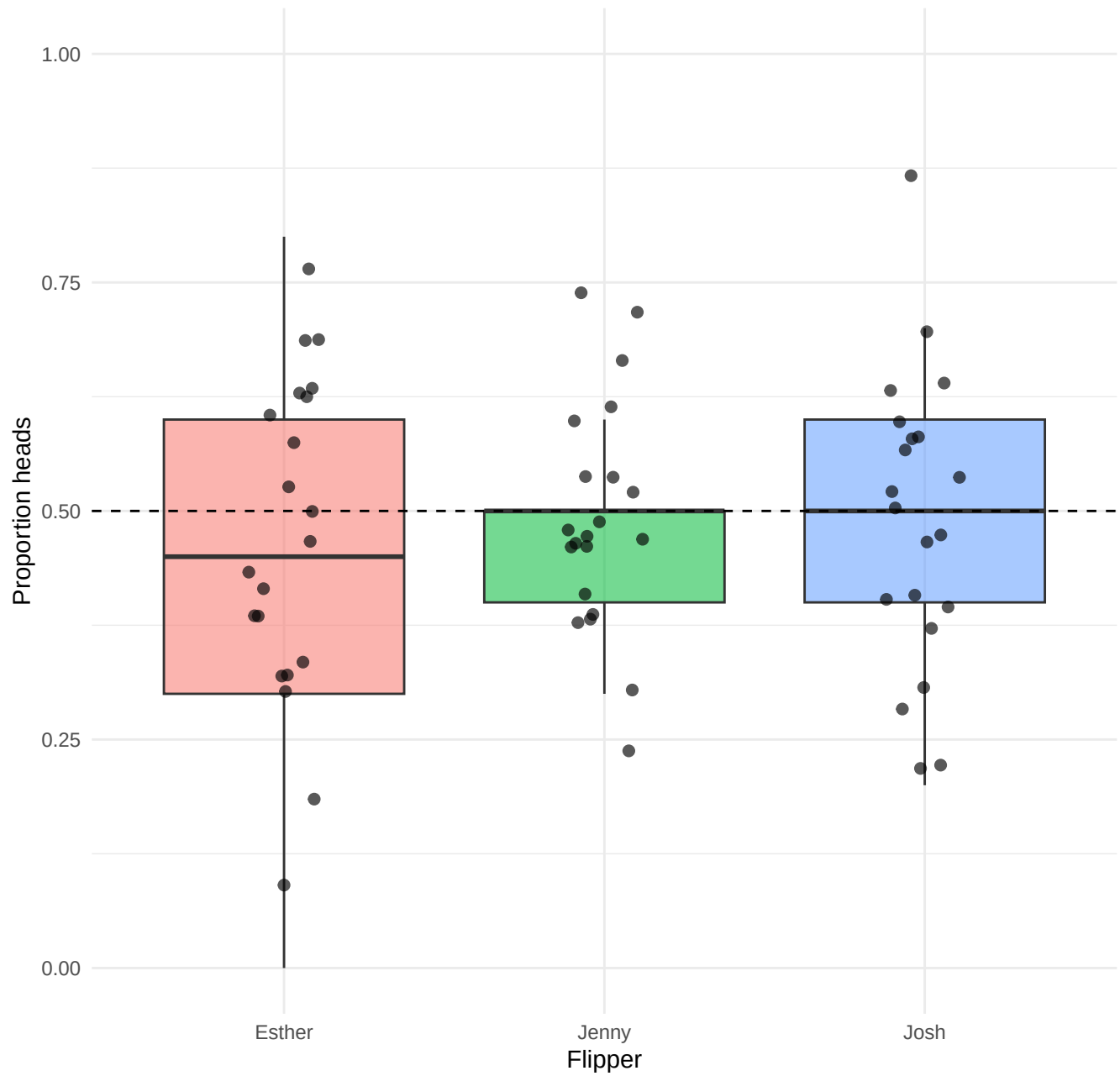
Nuisance-factor check by flipper
