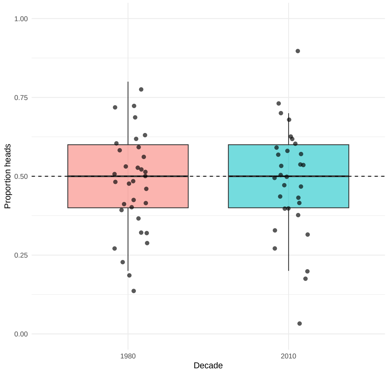
Nuisance-factor check by decade
