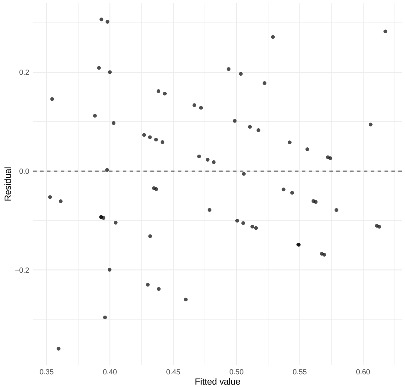
Residuals versus fitted values
