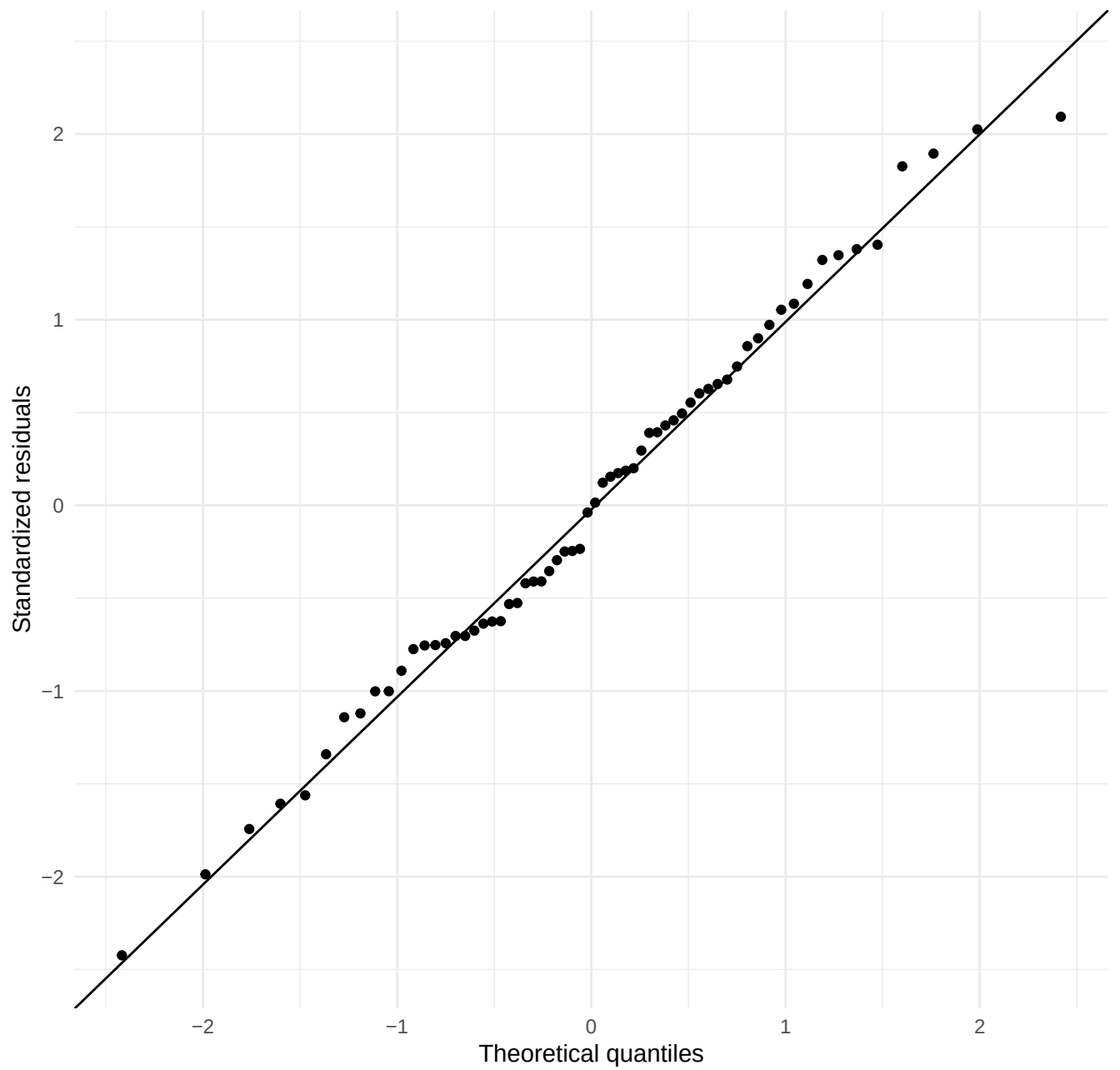
Normal Q-Q plot of model residuals
