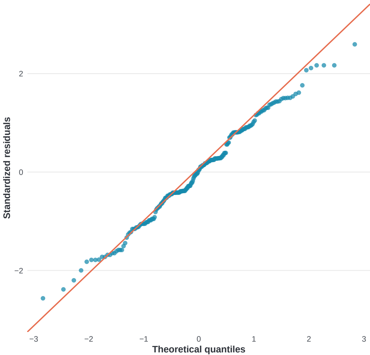
Normal Q-Q plot of model residuals
