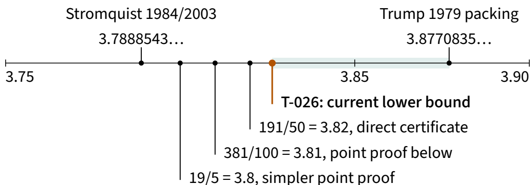
Figure 3. Bounds on s(11) . The shaded band is the gap left by the certificates explained here. At the current lower bound the gap is 0.0506361... wide, down from 0.0882292... at Stromquist's bound.
