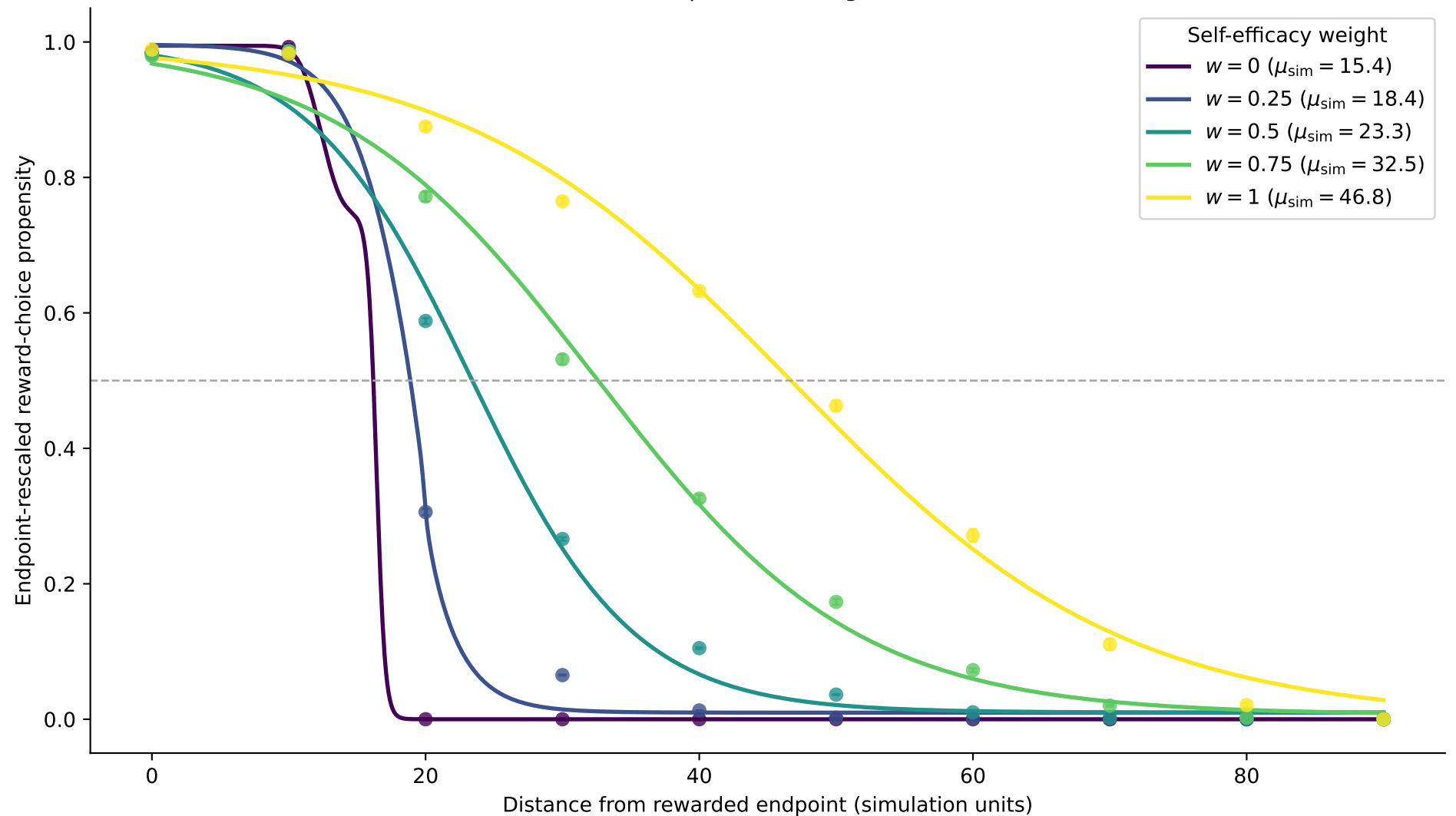
Model-implied choice gradients
