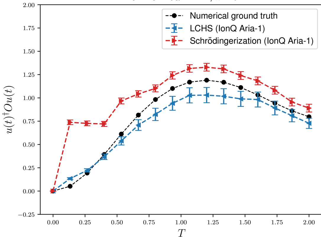
Non-Hermitian TFIM, n = 3
