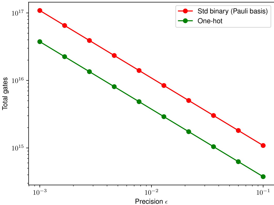
Estimated gate counts for simulating non-separable 2D advection equation
