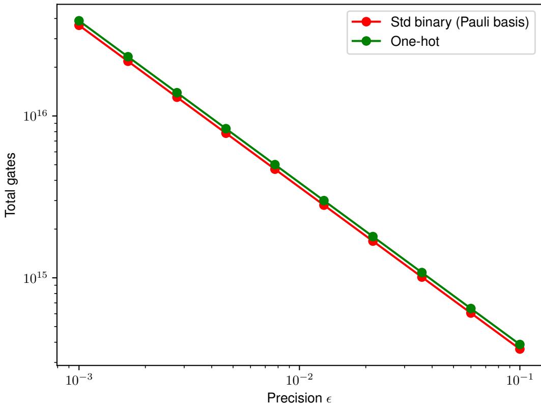
Estimated gate counts for simulating 1D nonlinear PDE
