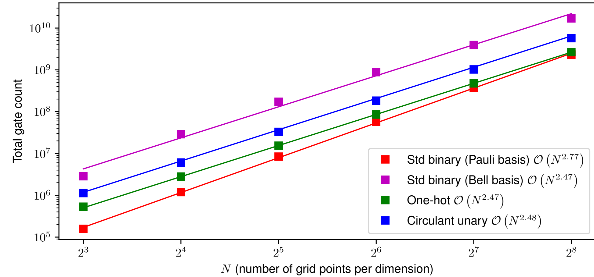
Resource analysis for 2D advection equation w/ upwind scheme
