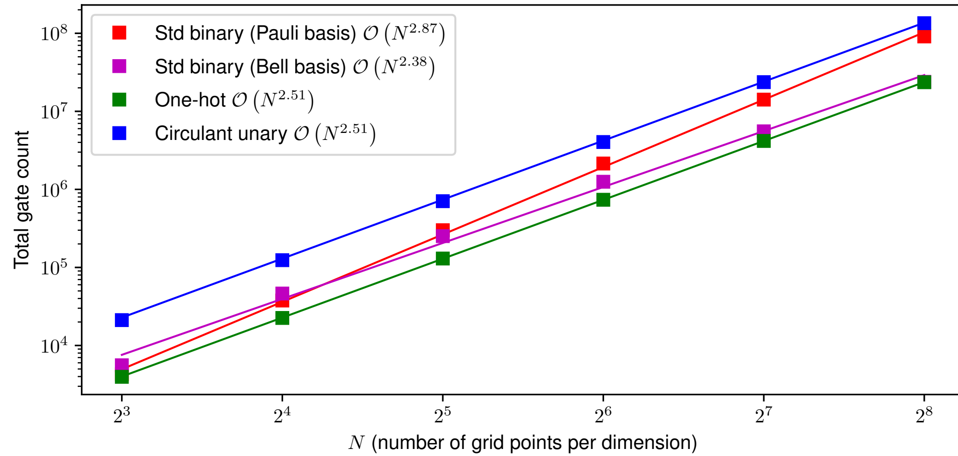
Resource analysis for 2D advection equation w/ centered differences
