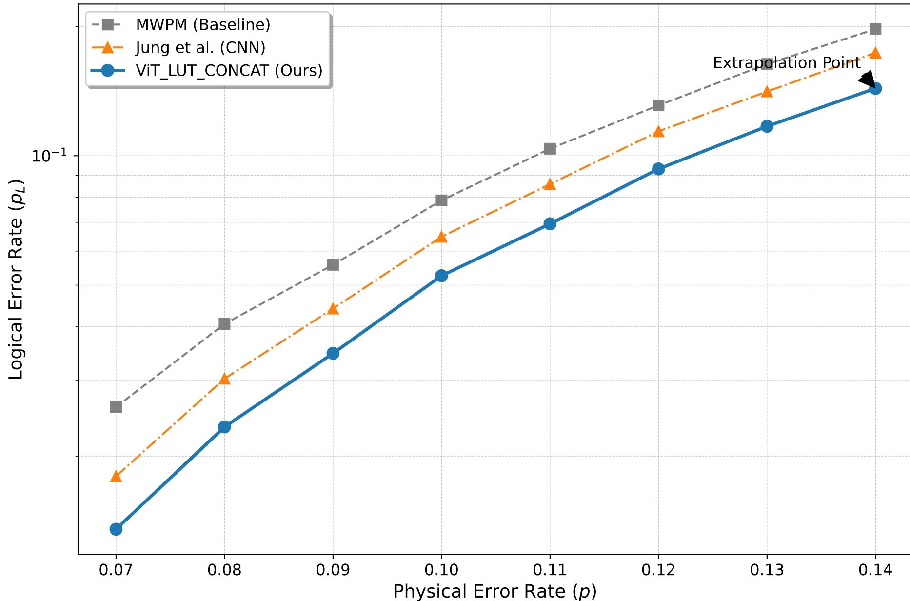
Decoding Performance Comparison ( L = 7 , Depolarizing)
