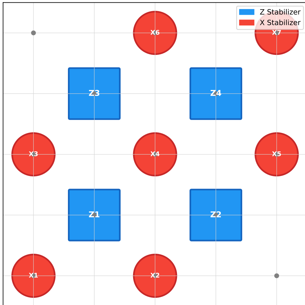
Surface Code (L=3) Stabilizer Layout
