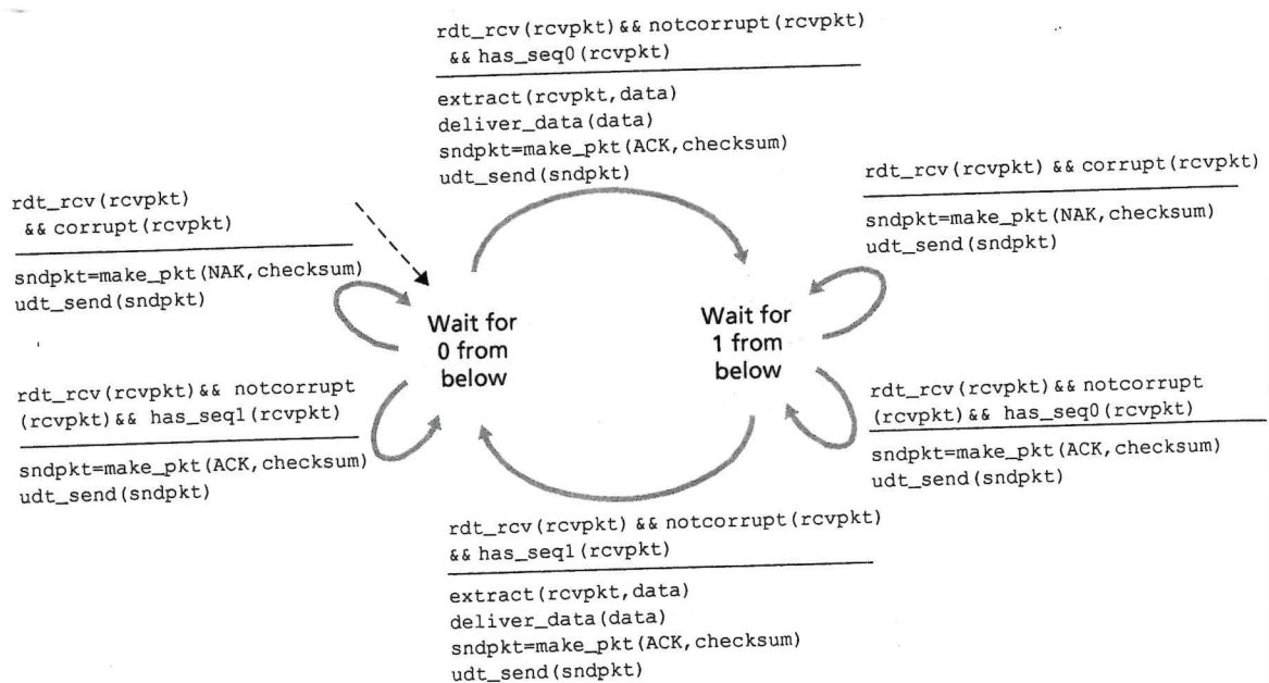
Figure 3.12 ♦ rdt2.1 receiver
