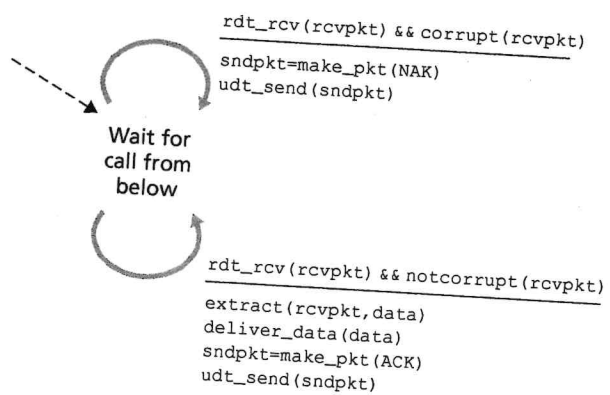
b. rdt2.0: receiving side
