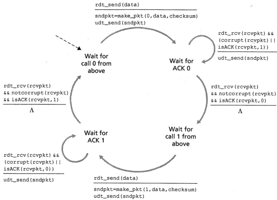
Figure 3.13 ♦ rdt2.2 sender
