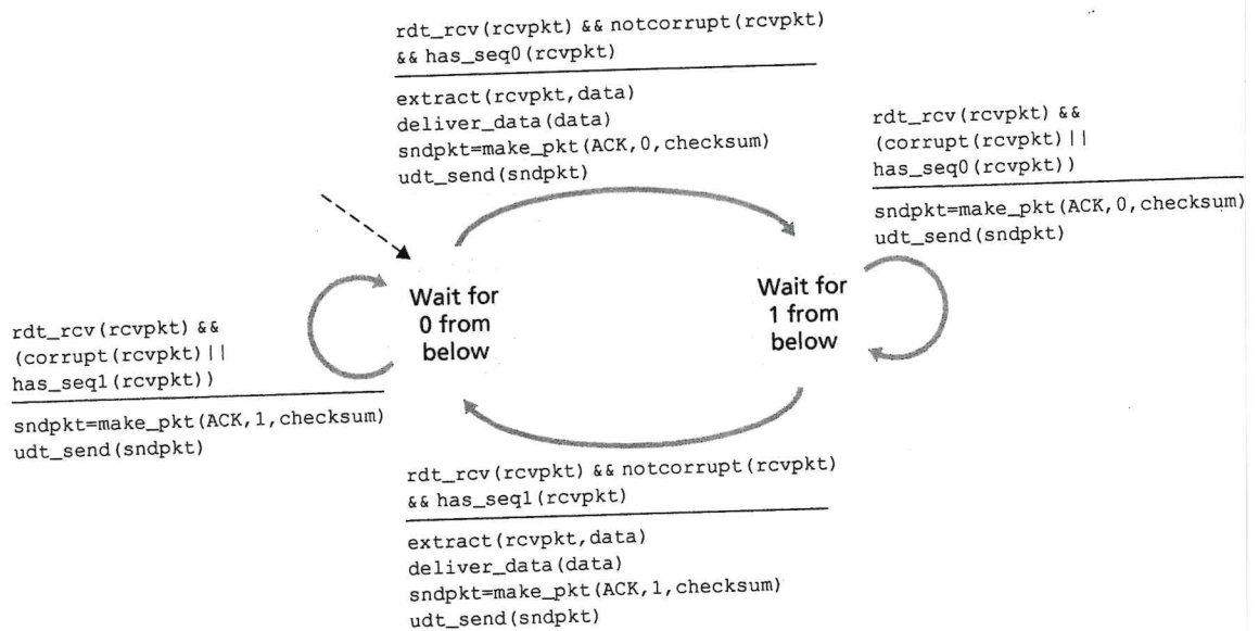
Figure 3.14 ♦ rdt2.2 receiver
