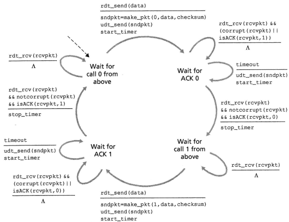
Figure 3.15 ♦ rdt3.0 sender
