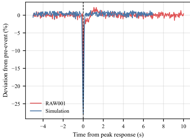
Voltage Magnitude Response
