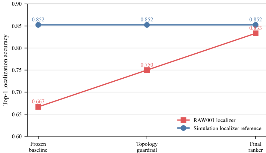
Localization Model Promotion Curve
