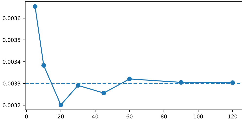
figure07_severity_posterior
