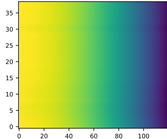
truth angle
