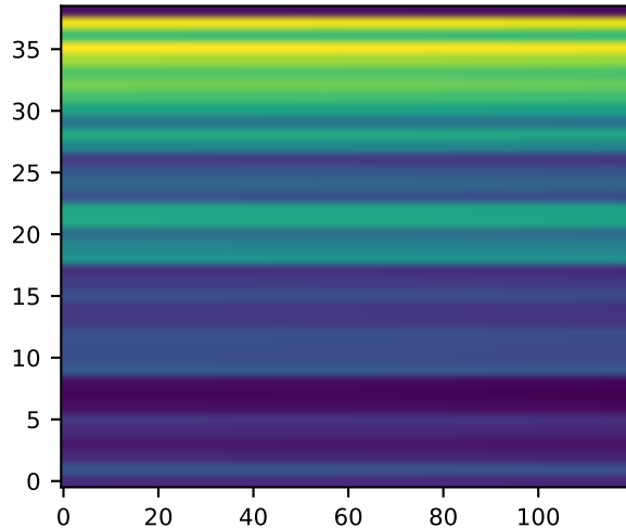
BMA angle
