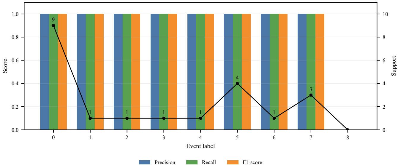
Per-Class Event Classification Metrics
