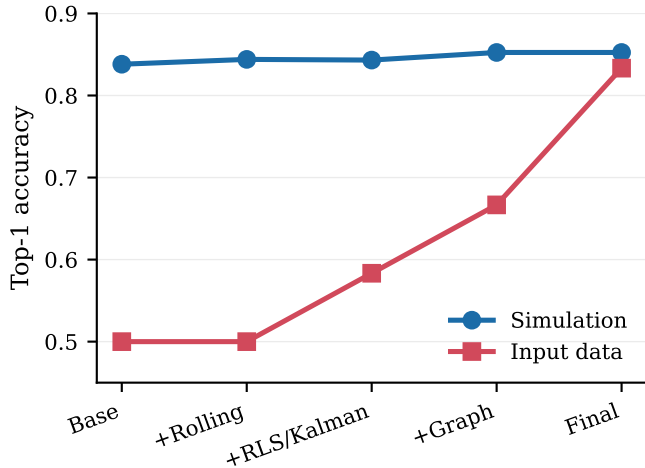
Localizer Validation Curve
