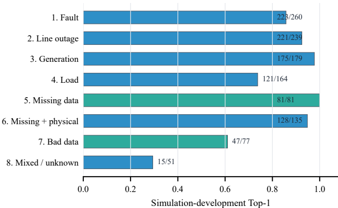
(a) Event-level exact localization
