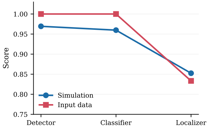
Primary Metric by Task
