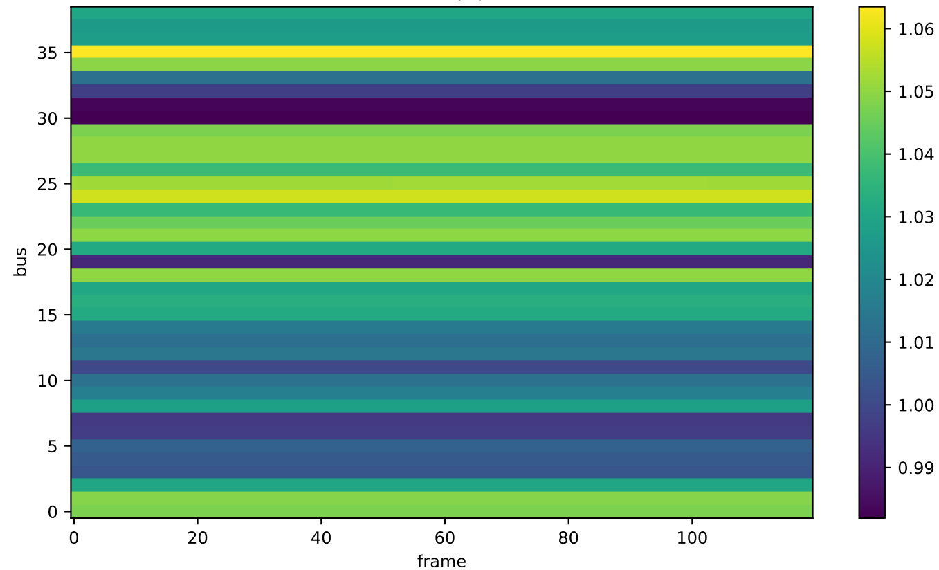
truth |V|
