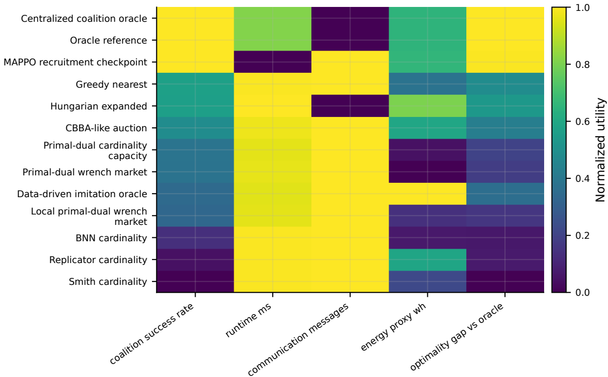
SP1 coalition recruitment: normalized metric matrix
