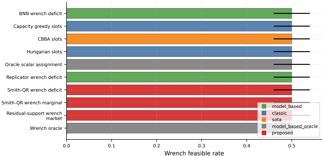
SP3 wrench feasibility: method ranking
