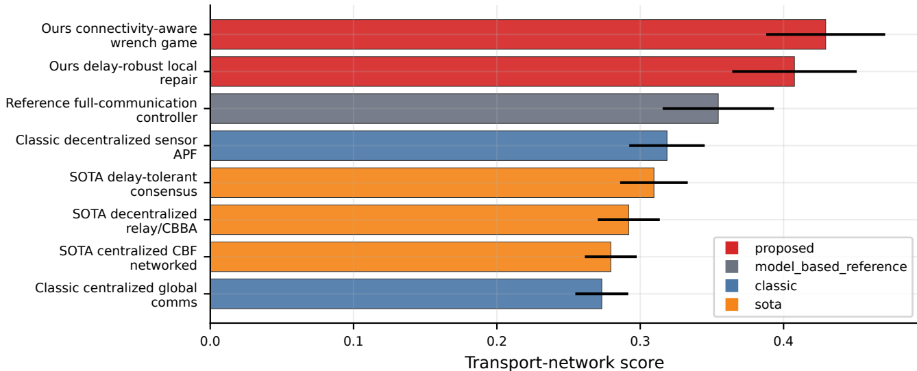
SP7 communication robustness: method ranking
