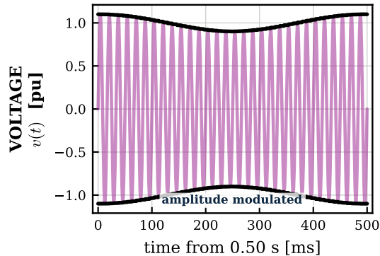
C Modulation: AM
