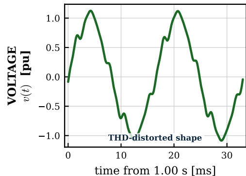
Harmonic distortion
