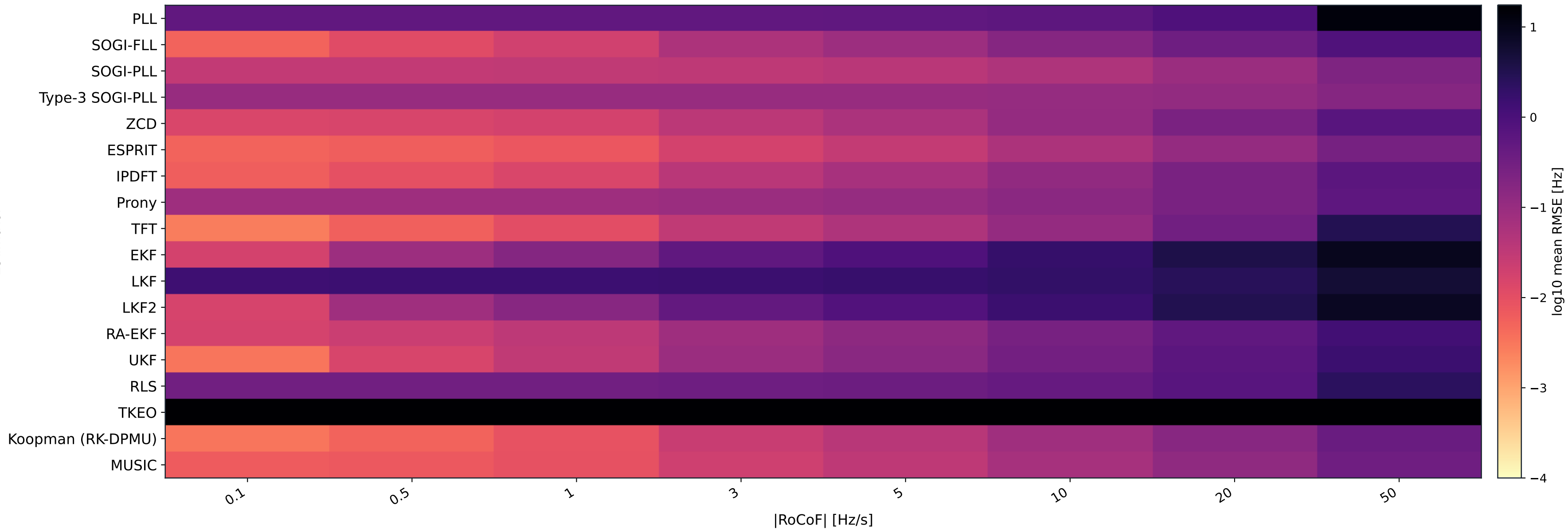
RoCoF method stress map
