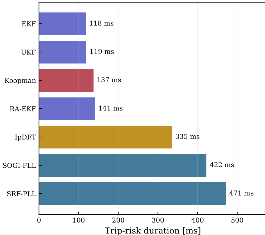
Scenario E: IBR multi-event
