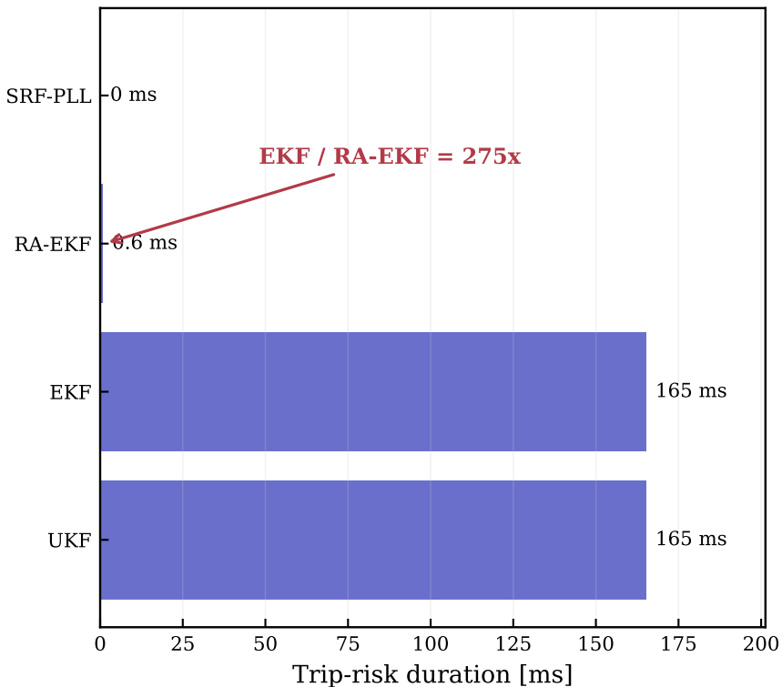
Scenario D: composite islanding
