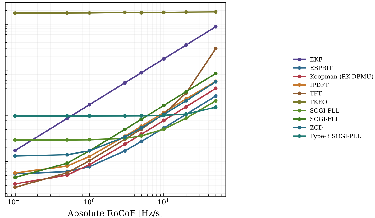
RoCoF ramp
