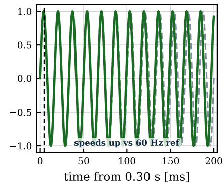
B Frequency ramp
