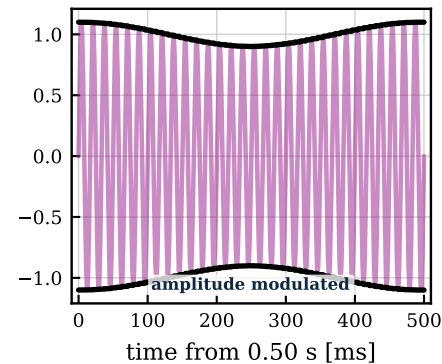
C Modulation: AM
