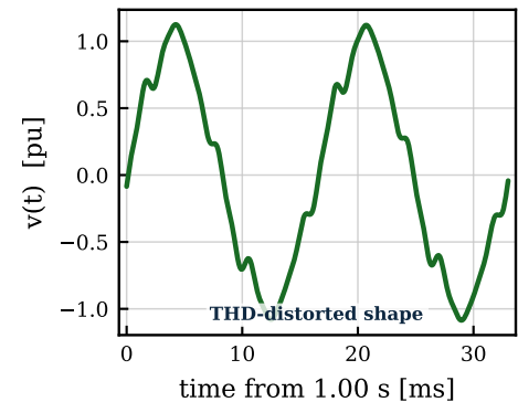
Harmonic distortion
