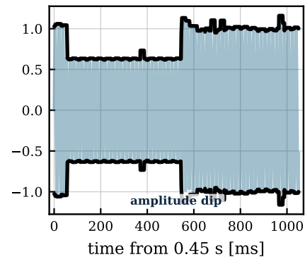
Power-imbalance ringdown
