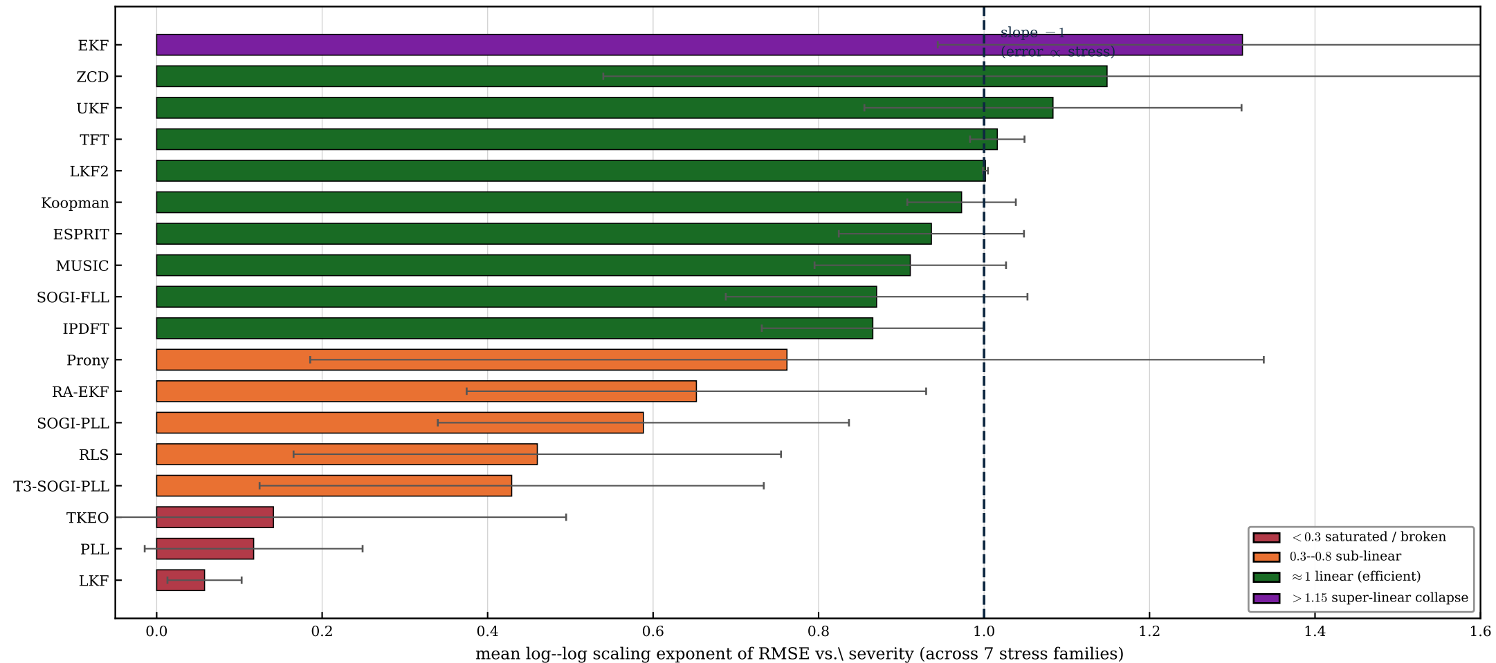
How error grows with stress: the scaling exponent classifies estimators
