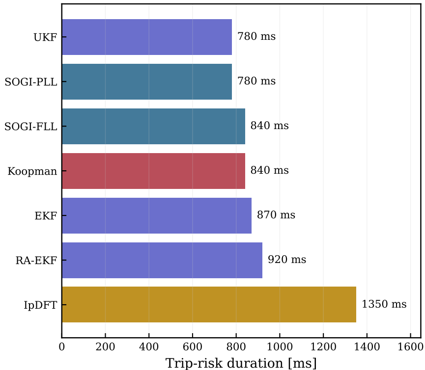
Scenario E: IBR multi-event
