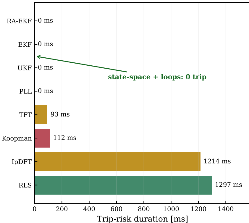
Scenario D: phase jump (NERC +60°)
