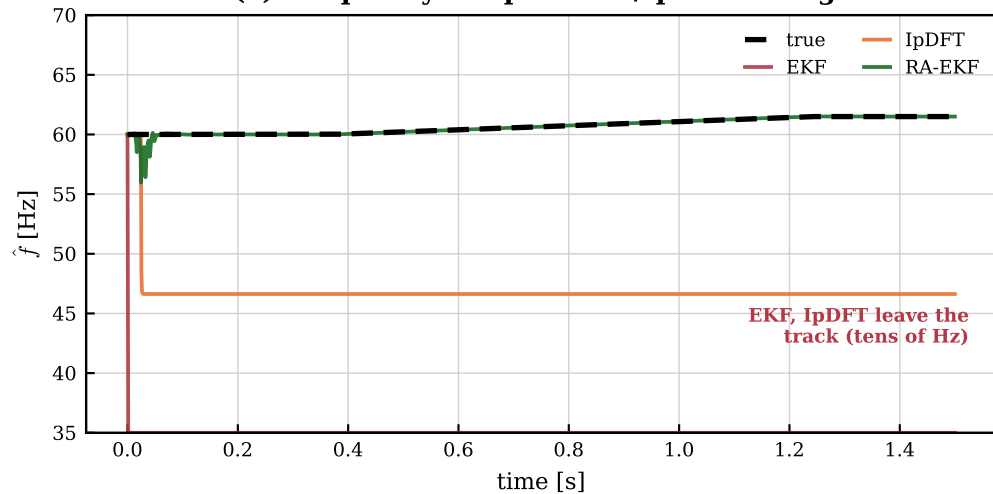
(a) Frequency ramp --- EKF/IpDFT diverge
