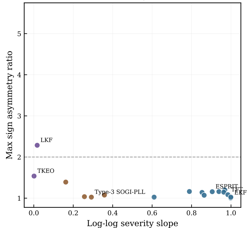
Frequency step
