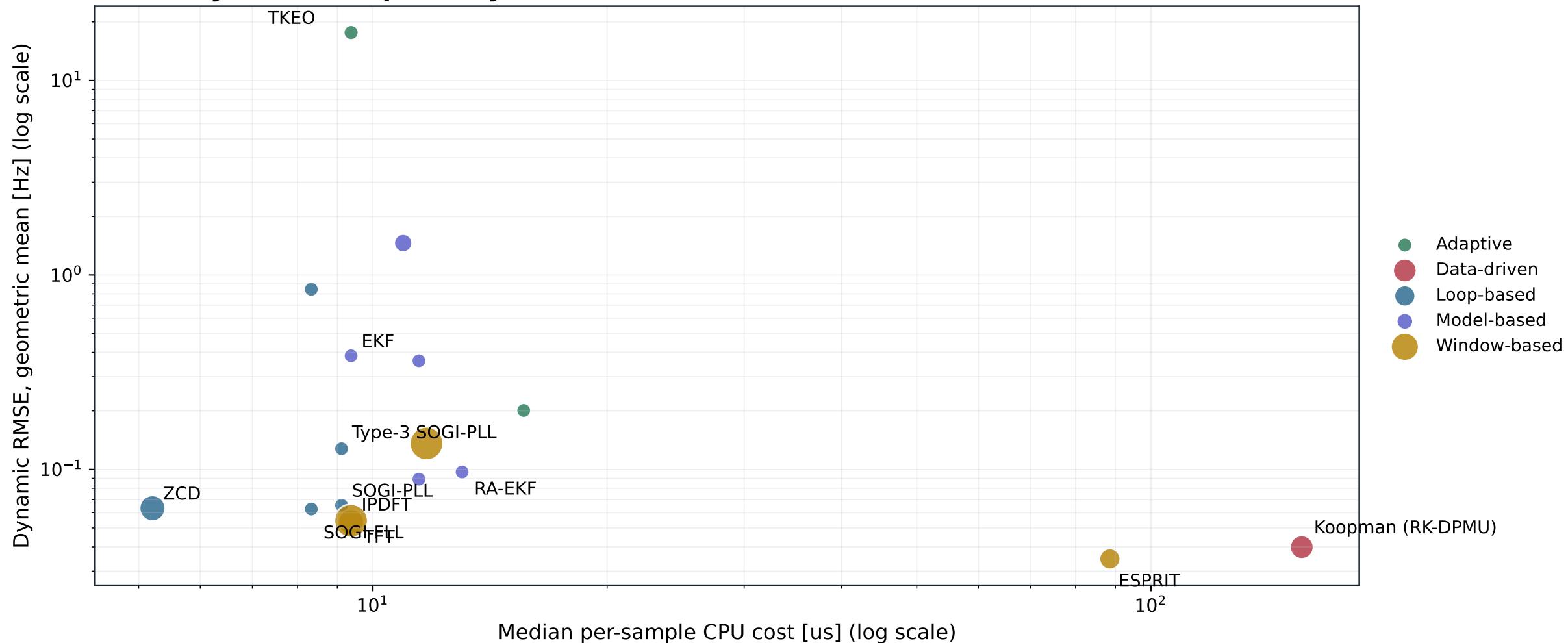
Accuracy costs compute: dynamic stress Pareto view
