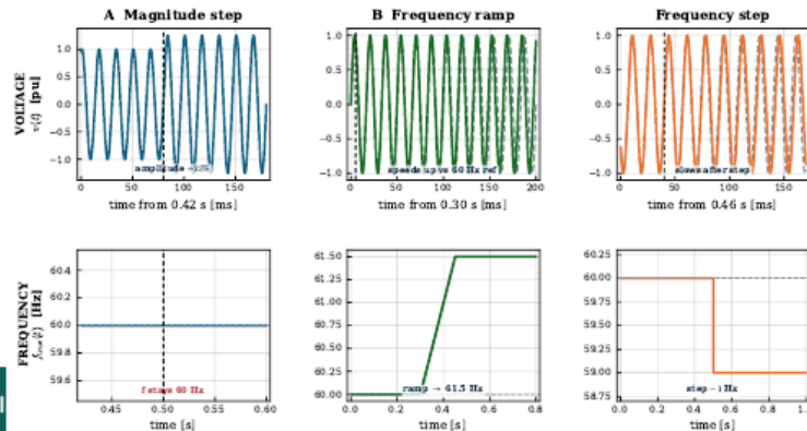
Standard stresses (1 of 2): VOLTAGE v(t) on top, true FREQUENCY f(t) below
