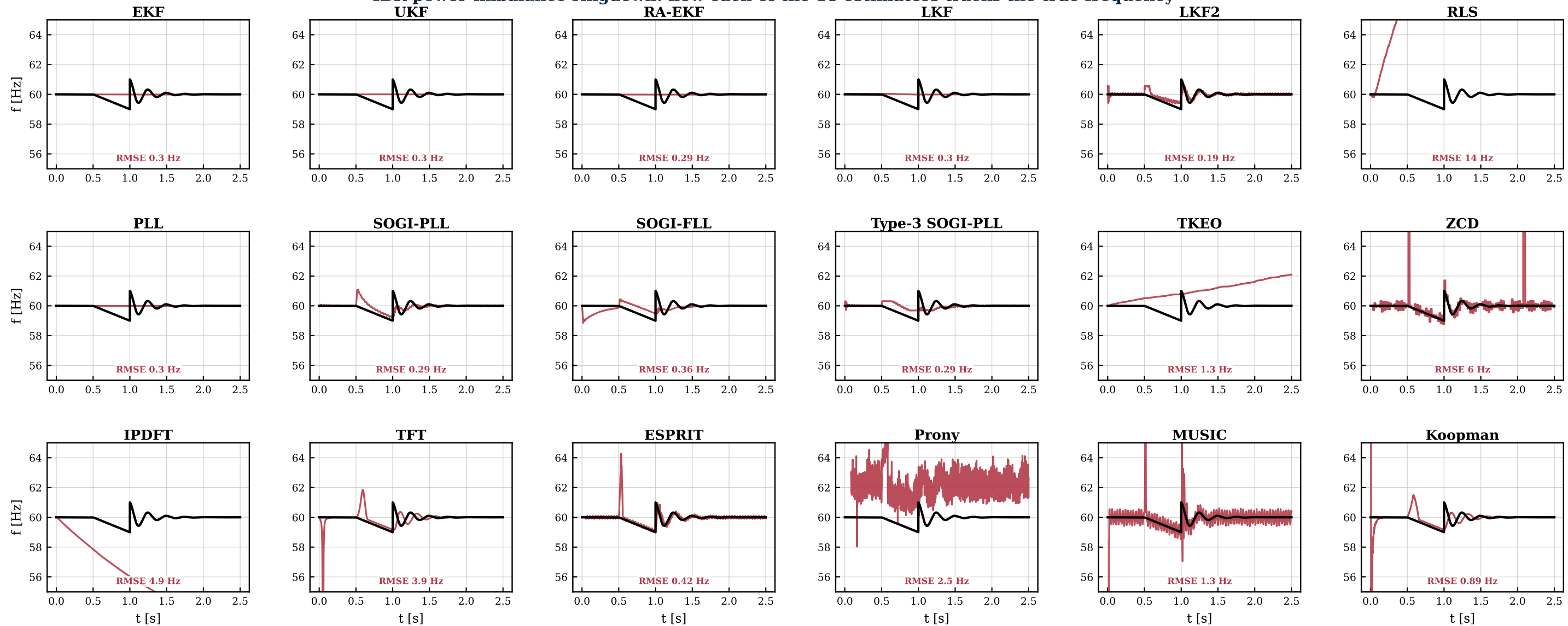
— true frequency f(t) — estimated \hat{f}(t) IBR power-imbalance ringdown: how each of the 18 estimators tracks the true frequency
