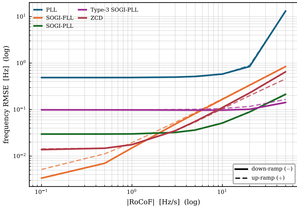
Loop-based: RMSE vs |RoCoF|, down (solid) vs up (dashed)
