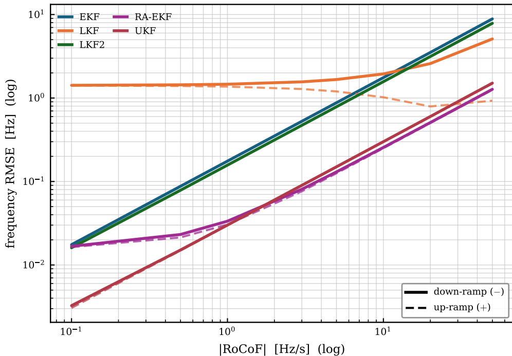
Model-based: RMSE vs |RoCoF|, down (solid) vs up (dashed)
