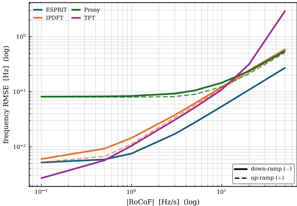
Window/spectral: RMSE vs |RoCoF|, down (solid) vs up (dashed)
