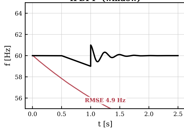
IPDFT (window)
