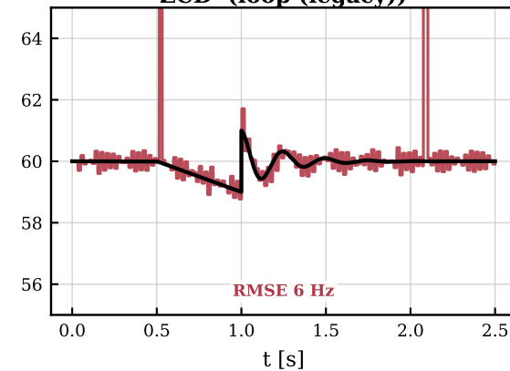
ZCD (loop (legacy))
