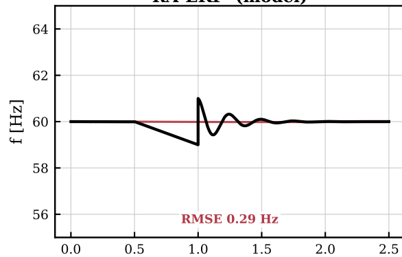
RA-EKF (model)
