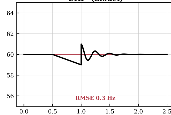
UKF (model)
