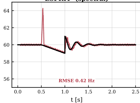
ESPRIT (spectral)
