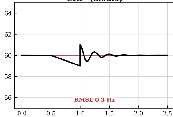
EKF (model)
