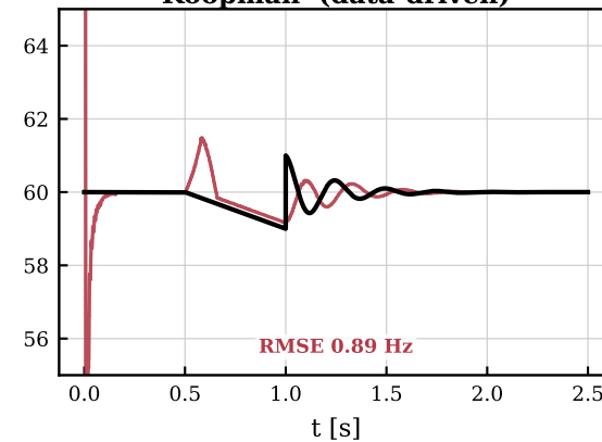
Koopman (data-driven)
