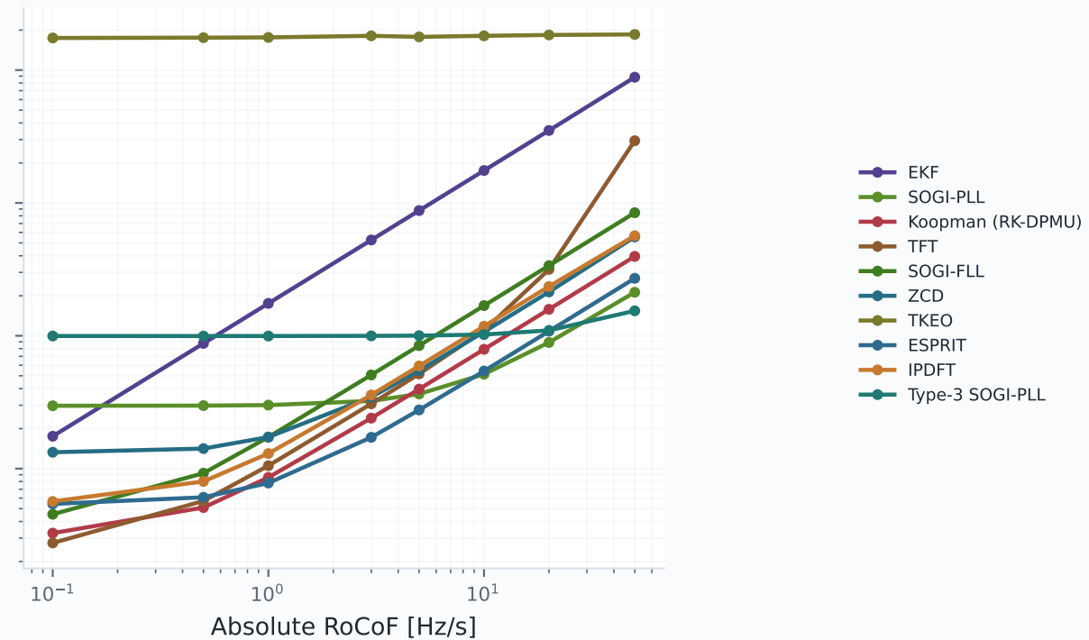
RoCoF ramp
