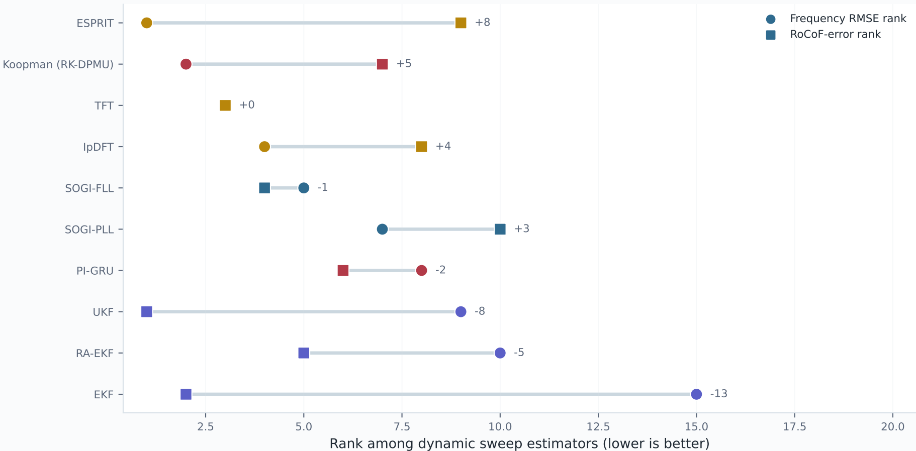
Metric choice changes the leaderboard: RMSE rank vs RoCoF-error rank
