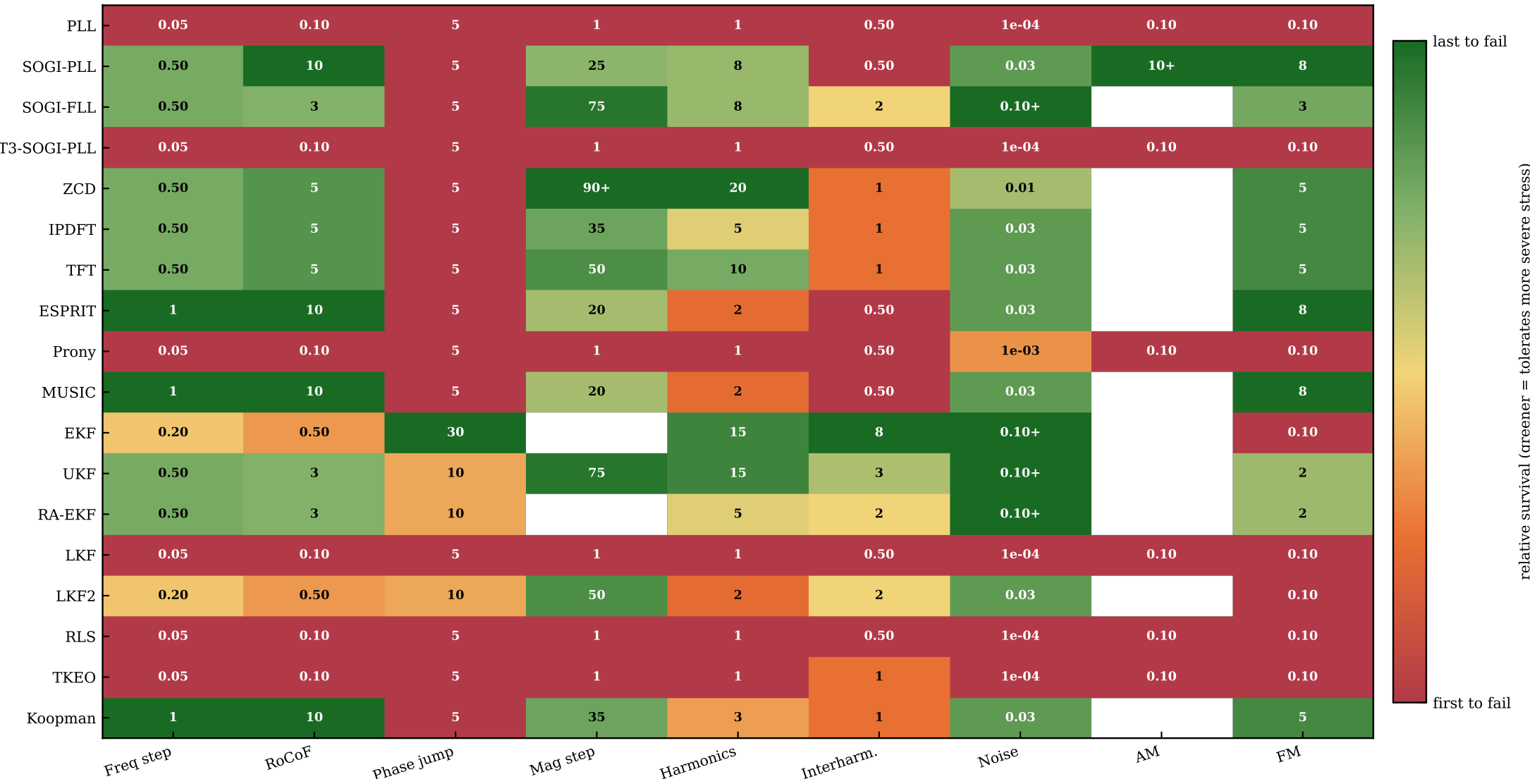
Safe-operating envelope: severity where frequency RMSE first exceeds 0.05 Hz
