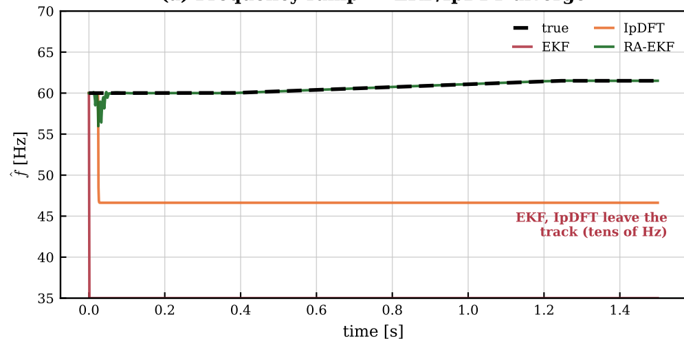
(a) Frequency ramp --- EKF/IpDFT diverge
