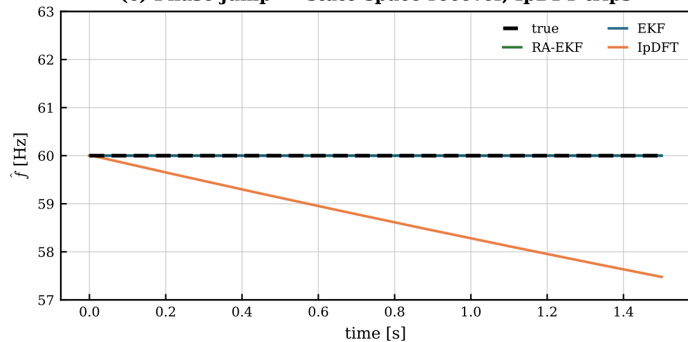
(c) Phase jump --- state-space recover, IpDFT trips
