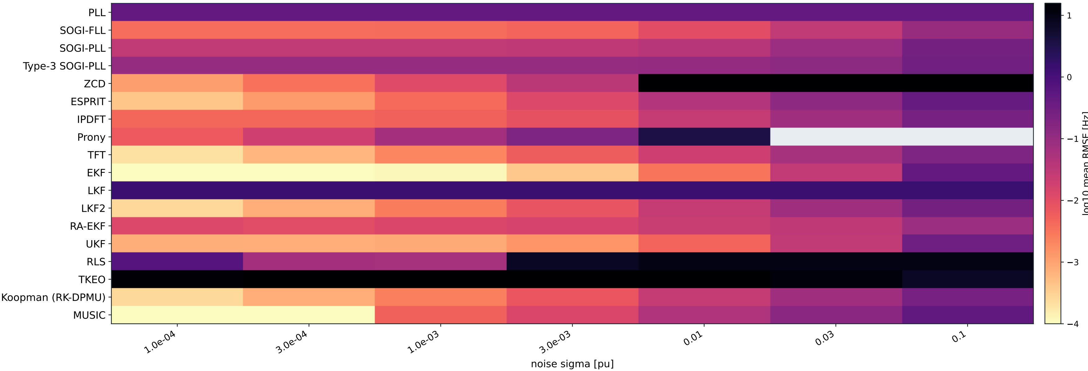
Broadband noise method stress map
