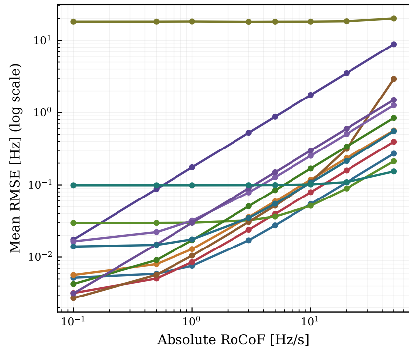
RoCoF ramp
