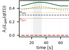
(c) realized vs. certified \lambda_2(\bar{L})
