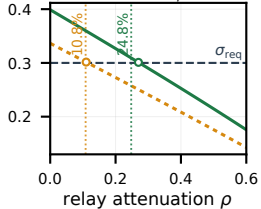
(b) certified \lambda_2(\bar{L}_\rho) budget
