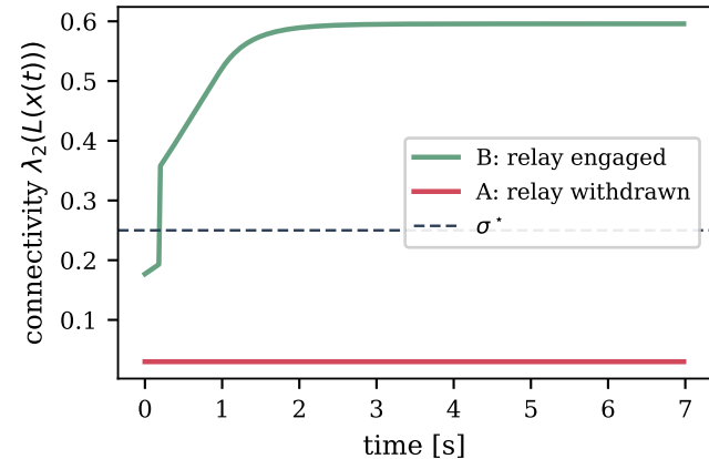
(a) induced connectivity
