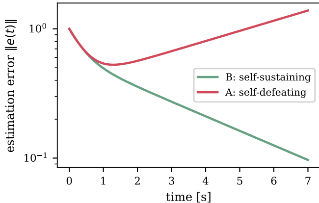
(b) threshold c m_F \lambda_2 > \vartheta^2
