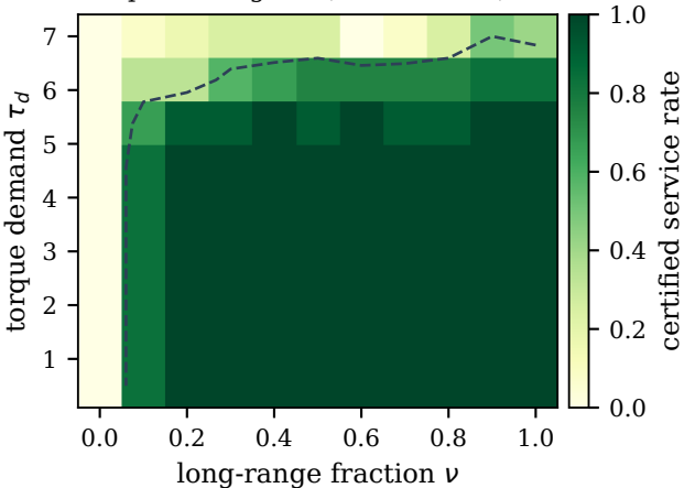
phase diagram (12 seeds/cell)
